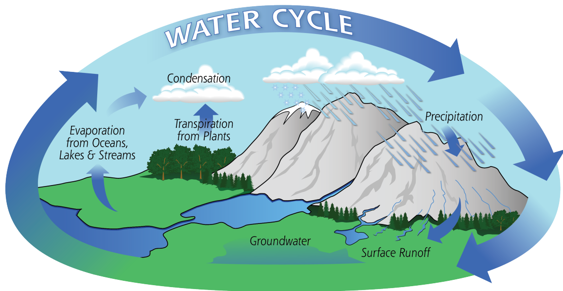
Figure 4. The Water (Hydrologic) Cycle.
